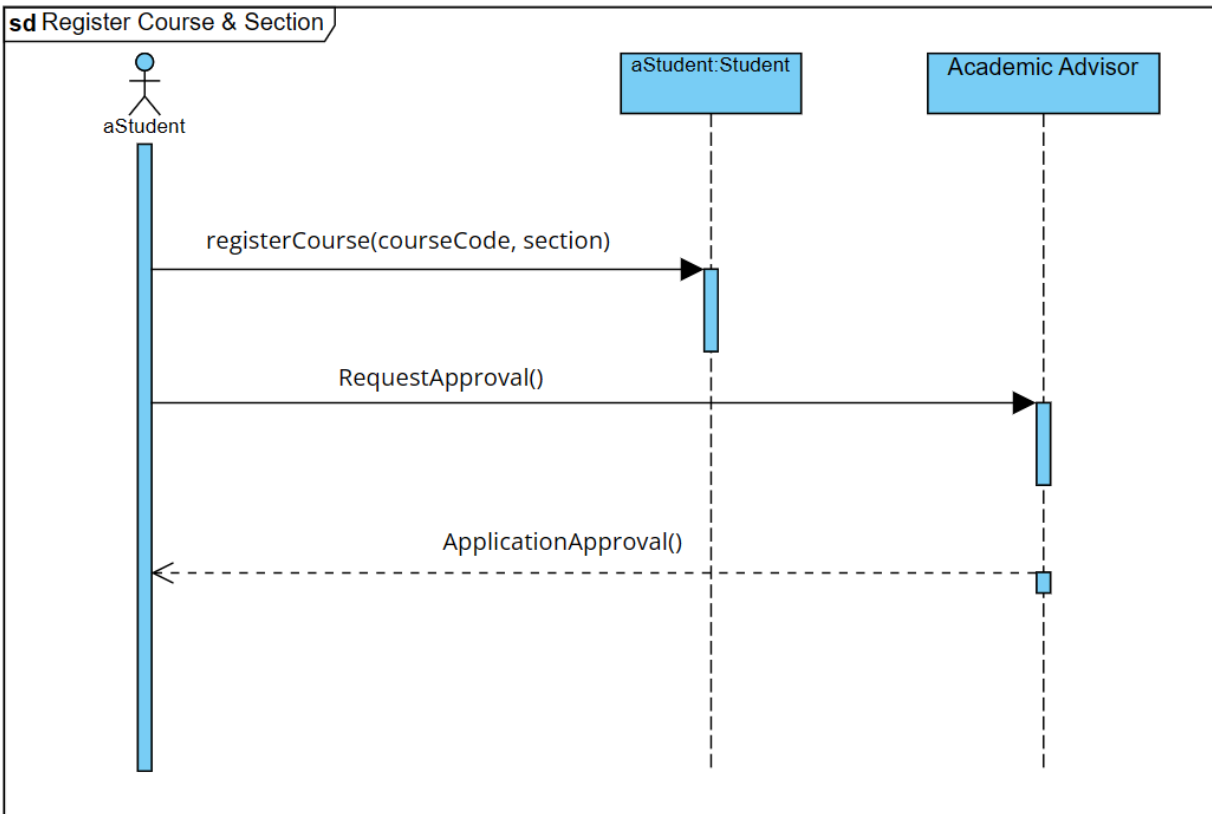
Figure 1.4.3 Use Case 1 : Sequence Diagram
