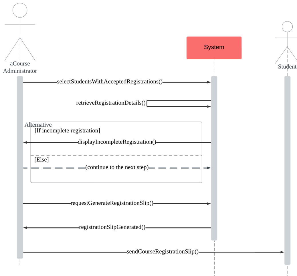
Figure 1.7.3 Use Case 5 : Sequence Diagram
