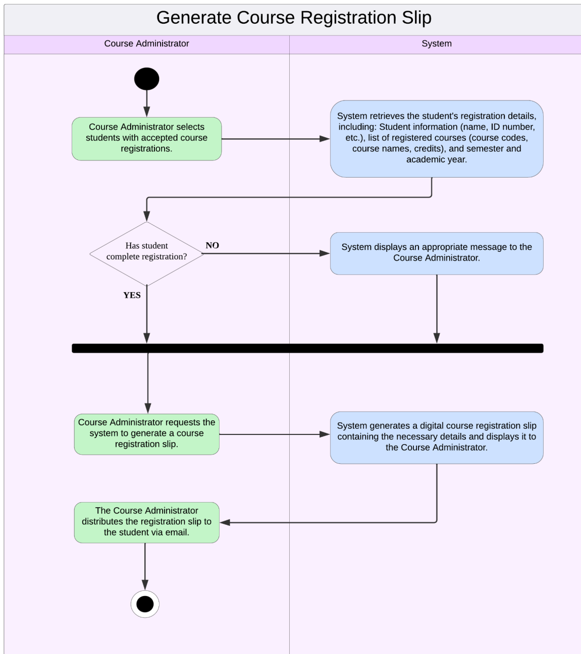
Figure 1.7.2 Use Case 4 : Activity Diagram
