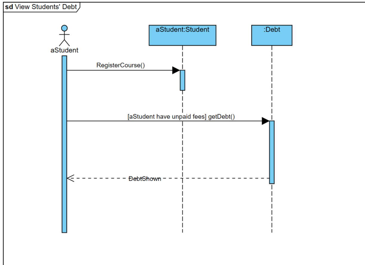
Figure 1.3.3 Use Case 2 : Sequence Diagram
