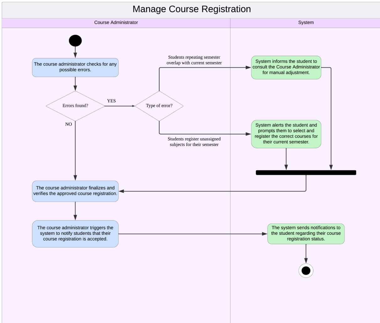
Figure 1.6.2 Use Case 4 : Activity Diagram
