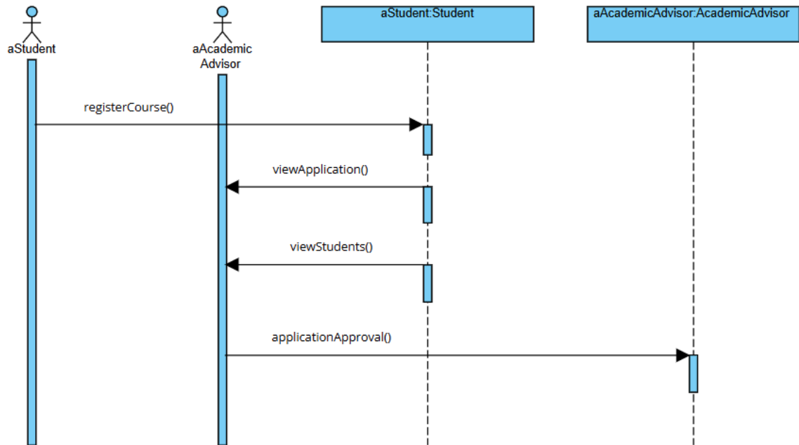
Figure 1.5.3 Use Case 3 : Sequence Diagram
