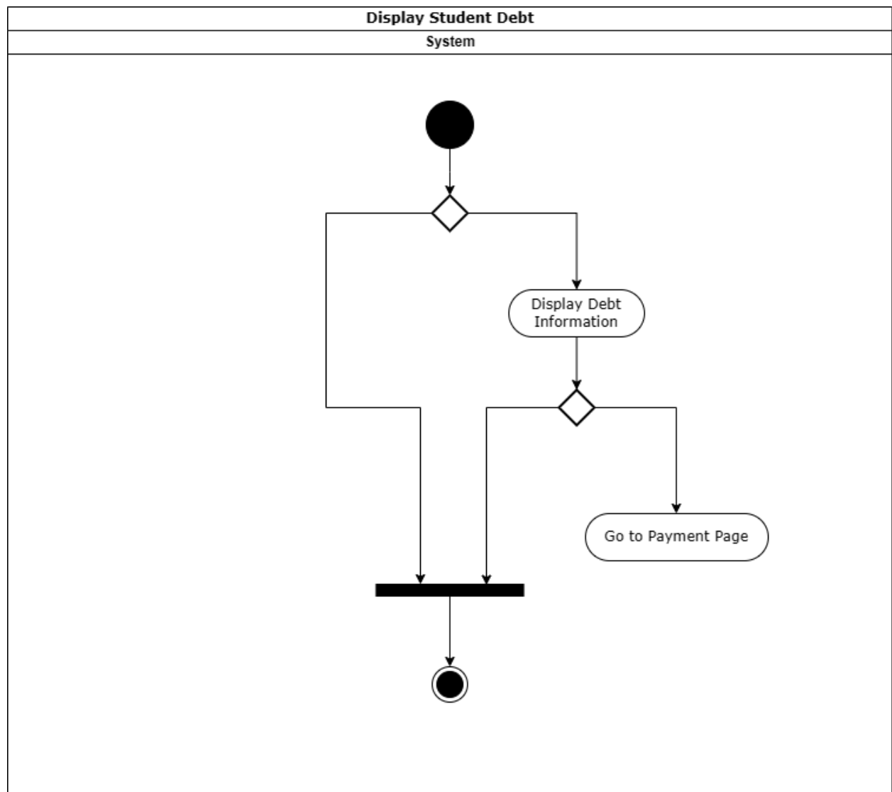
Figure 1.3.2 Use Case 2 : Activity Diagram
