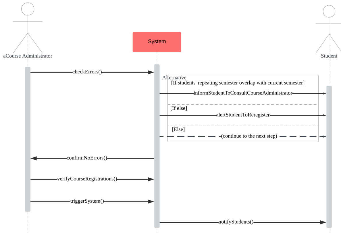
Figure 1.6.3 Use Case 4 : Sequence Diagram
