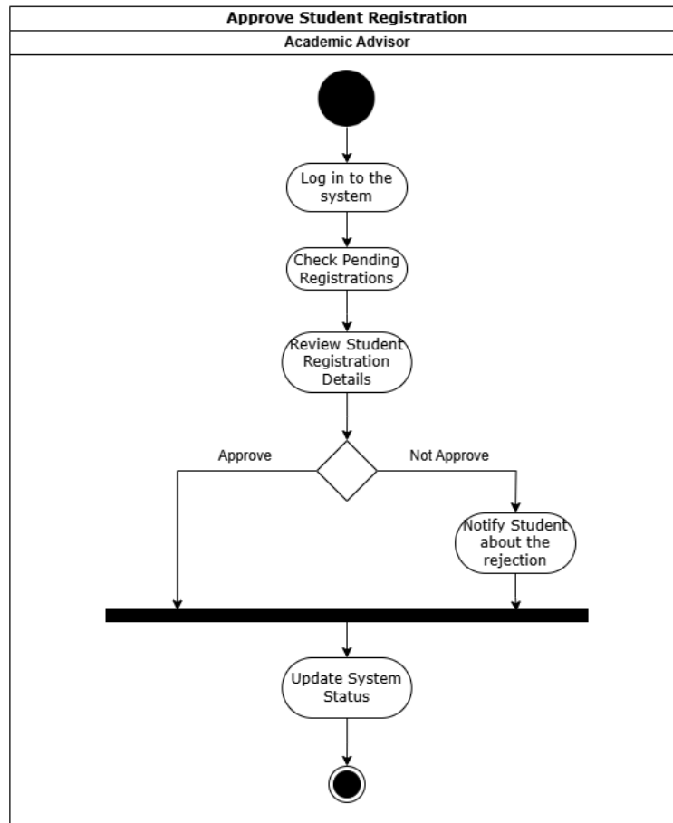
Figure 1.5.2 Use Case 3 : Activity Diagram
